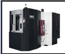
"New" OKK HM-500S, 20"x20" Twin Pallet, 40T, Coolant Thru, 12K RPM, 60 ATC, 30HP, Fanuc 180i. Stock Special!
